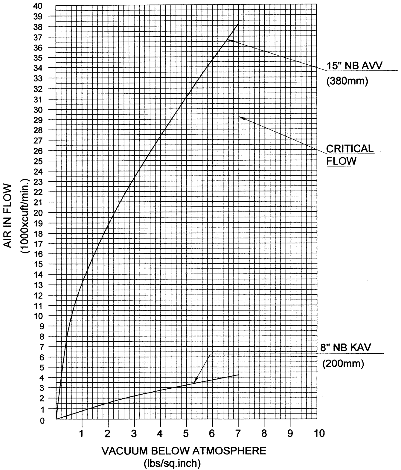
RELATIVE AIR INTAKE CAPACITY OF KINETIC AIR VALVE & ANTI VACUUM VALVE
